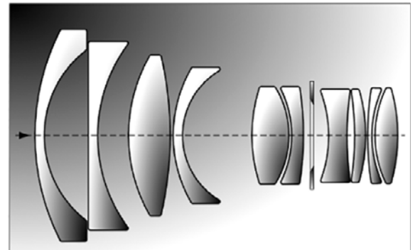
Fig. 4. High-end lens.
