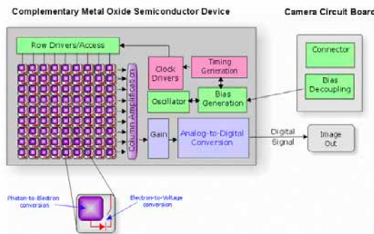
Fig. 8. CMOS Functional Diagram.
