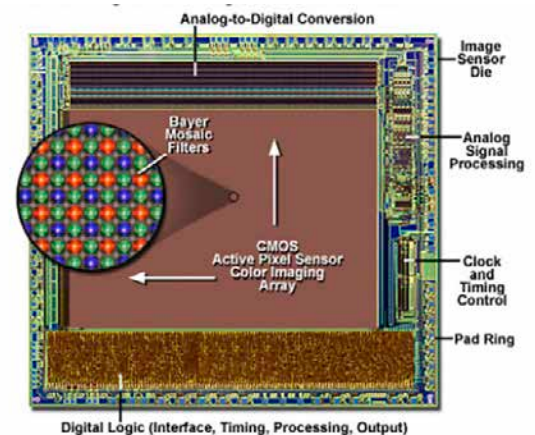
Fig. 7. CMOS Image Sensor Integrated Circuit Architecture.
