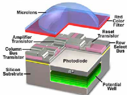
Fig. 6. CMOS PixelCell Anatomy.
