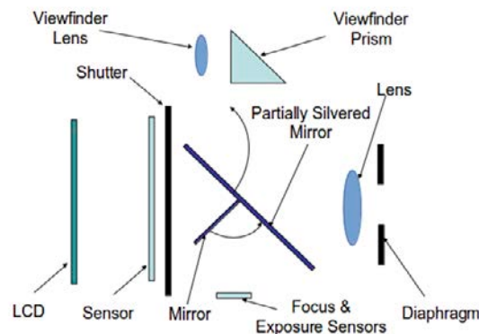
Fig. 3. Digital Single Lens Reflex Architecture.
